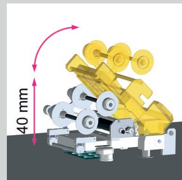
Vertical hinged opening system
