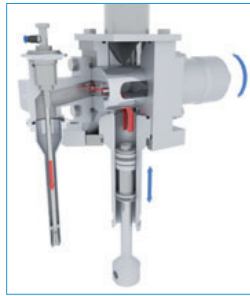
Filling system with optimized product flow and more effective easy to clean design
