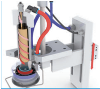
Sustainable energy savings with new state-of-the-art hot air cooling system
