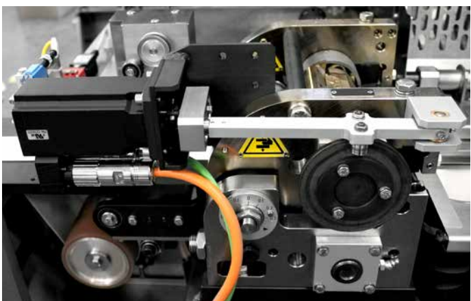
Servo-driven strip pack technology
