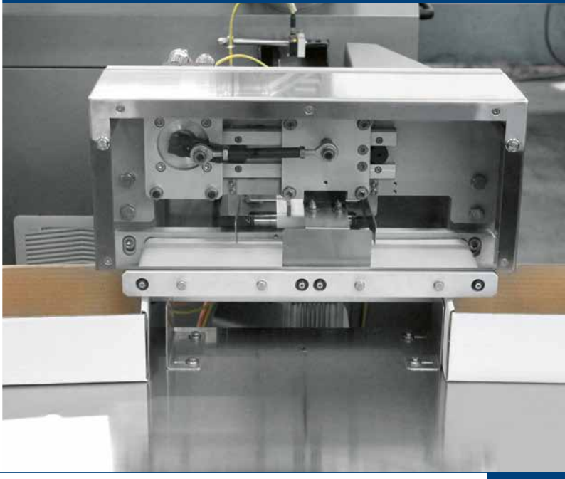
Servo-driven packs counting device
