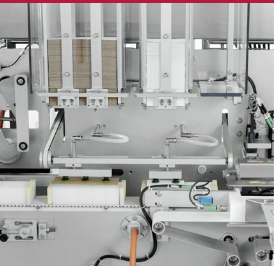
Interlayer and leaflet infeed
