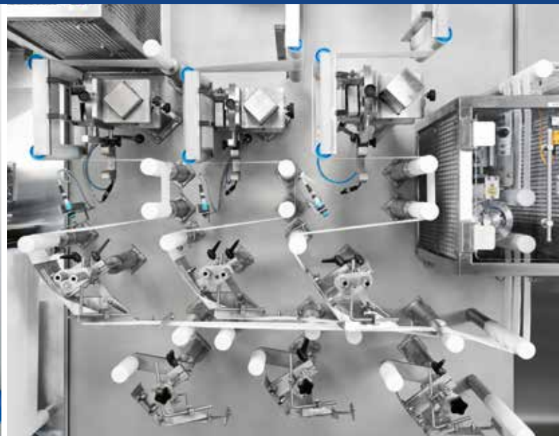
Extremely compact folding and wetting section complete with automatic edge guiding systems
