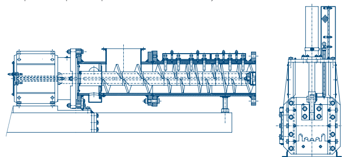
Feeder and insulated Conditioner with steamkit to be placed on top of the expander
