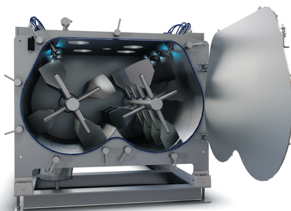
Each pop-up nozzle contains four customized air jets to clean the different surfaces.
