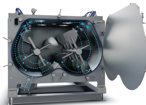
The air jets spread along the surfaces, blowing particles in the air which are then vacuumed through the outlet.
