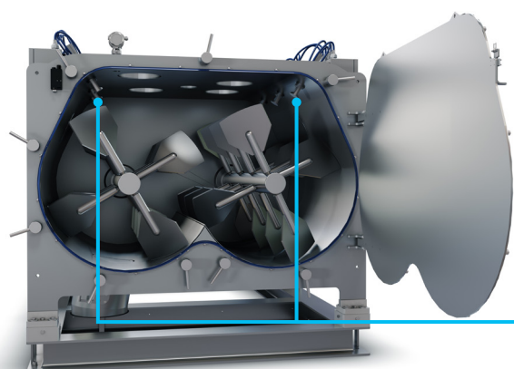
Pop-up nozzles are located on the top corners of the mixer's ceiling.
